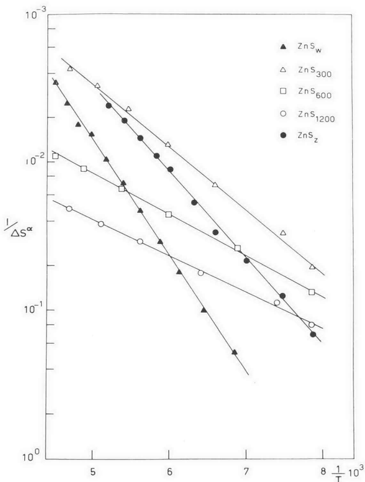
Fig. 3 - Plot of \ln(I/\Delta S^\alpha) versus 1/T for all the examined samples.
